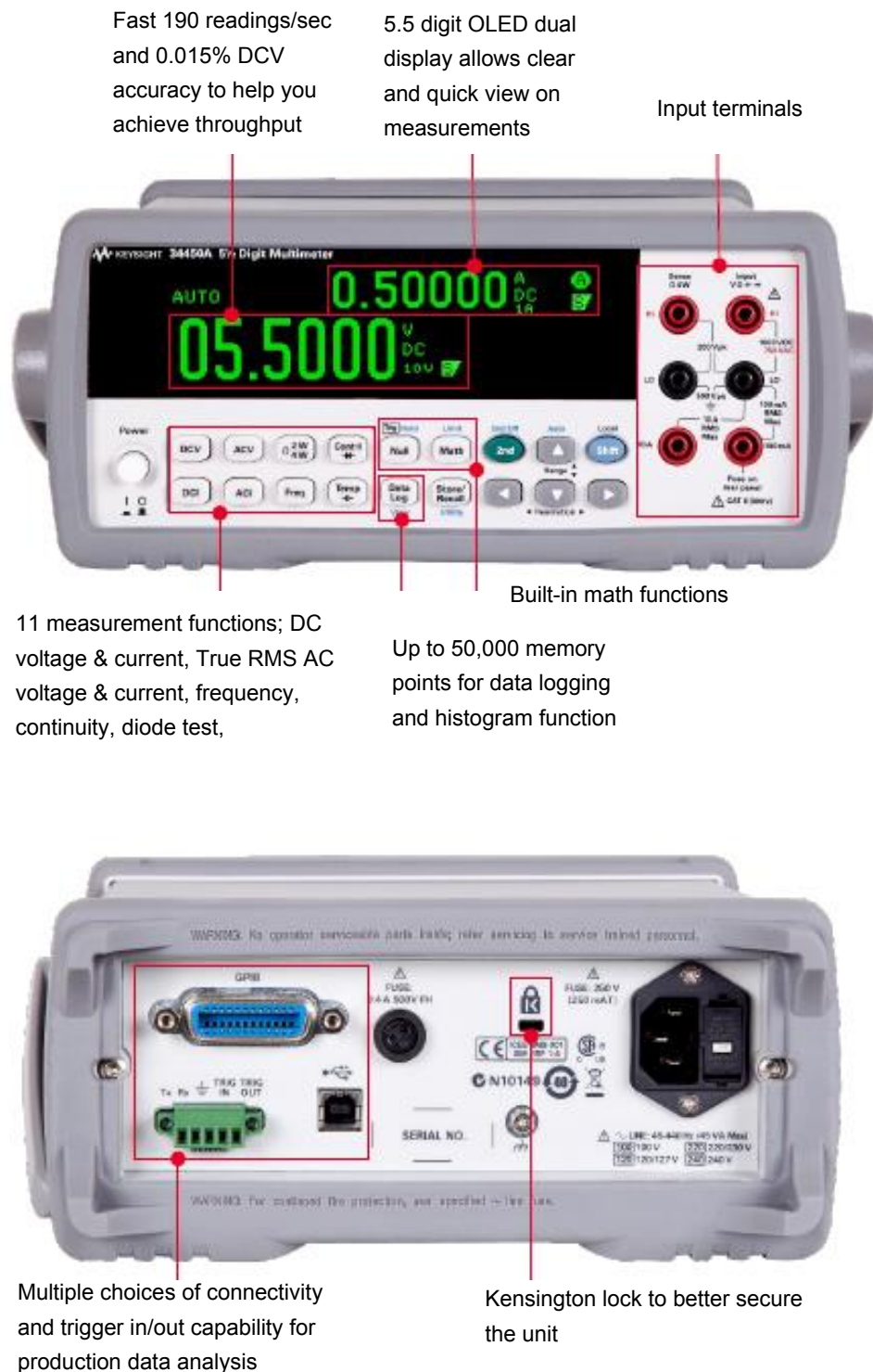
Figure 2. The front and rear view of 34450A
