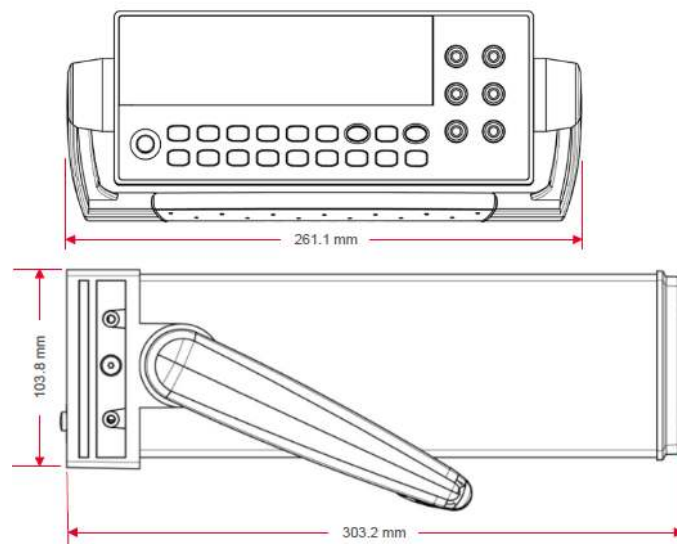
Figure 5. Product dimension
